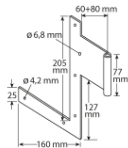
Standard-Winkelband
